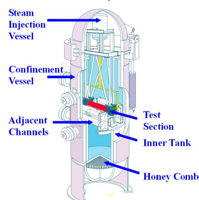
Former Molten Fuel Moderator Interaction Vessel (to be modified)
